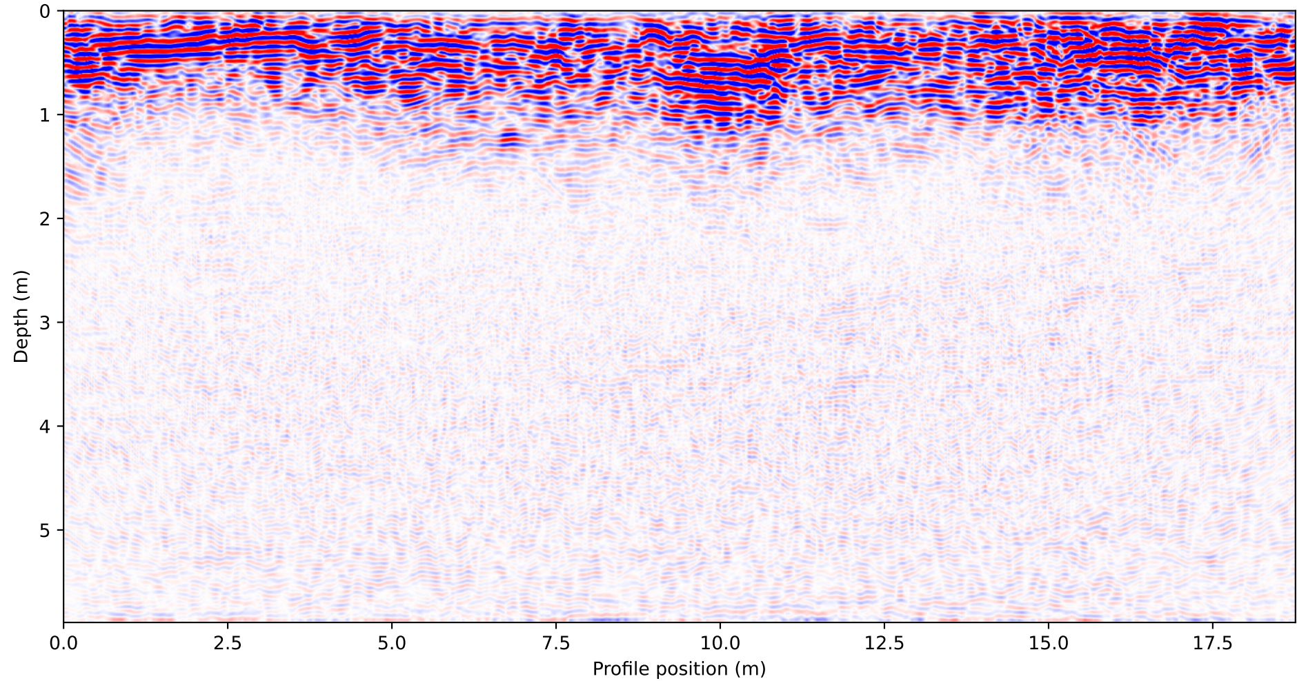
GPR Profile: line4.dt1
